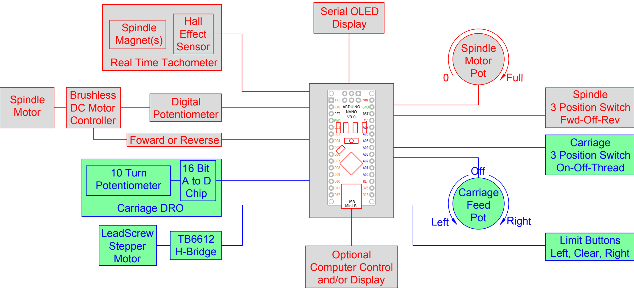
Concept Block Diagram For Arduino Control System for Taig Lathe
